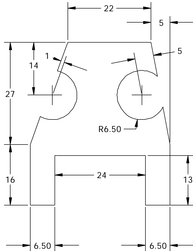
Dimensions (mm)
